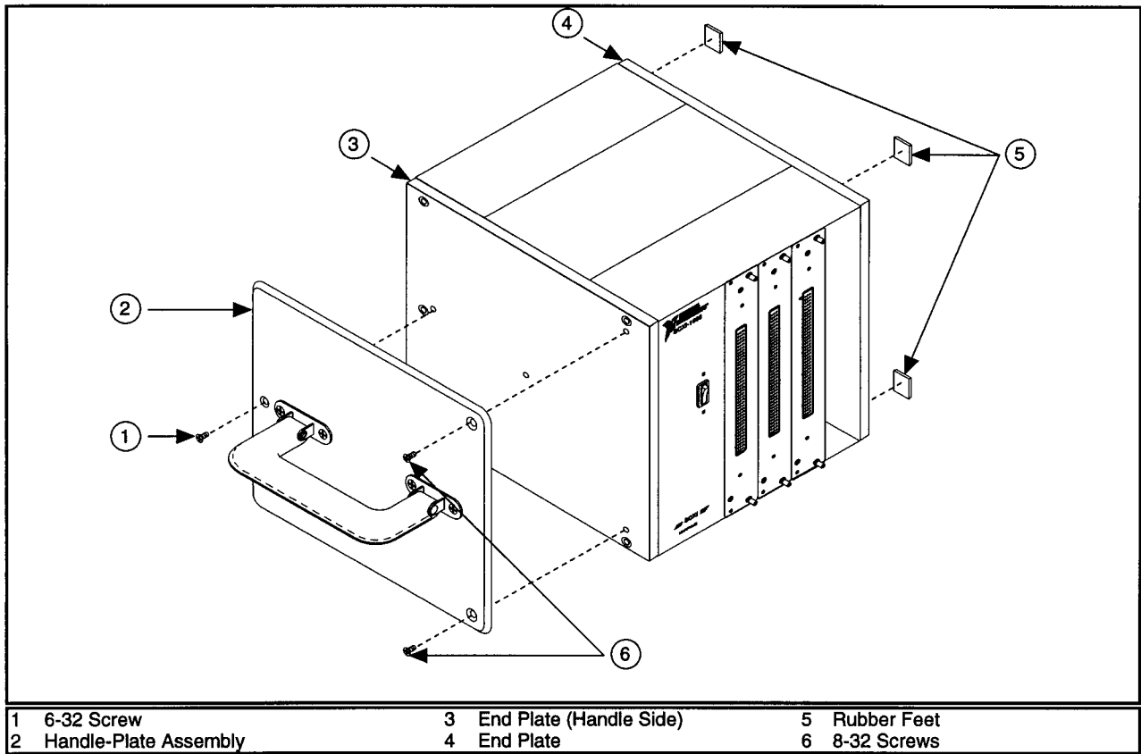
Figure 1. Connecting the Handle-Plate Assembly to the SCXI Chassis
